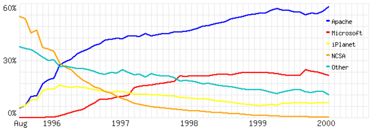
Figure 2-3. Web server software by Netcraft between 1995 and 2000.
